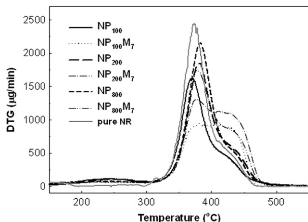
Fig. 13. DTG curves of pure NR, \text{NP}_x , and \text{NP}_x\text{M}_7 nanocomposites.
