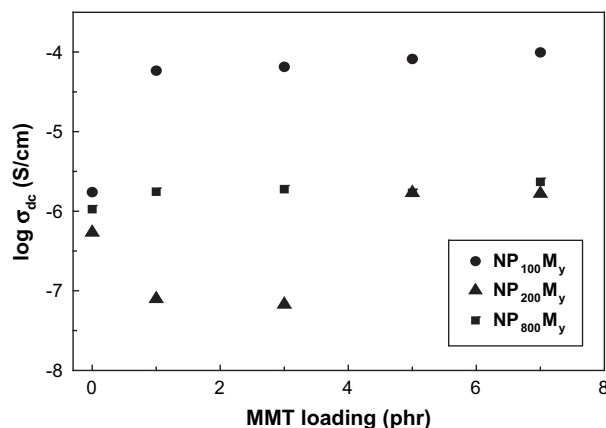
Fig. 8. Plot of the DC conductivity against clay loading of the nanocomposites.
