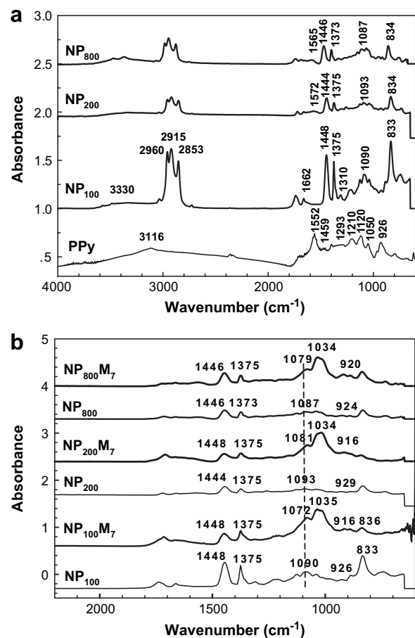
Fig. 6. FTIR spectra of (a) PPy and \text{NP}_x composites, and (b) \text{NP}_x and \text{NP}_x\text{M}_7 nanocomposites.
