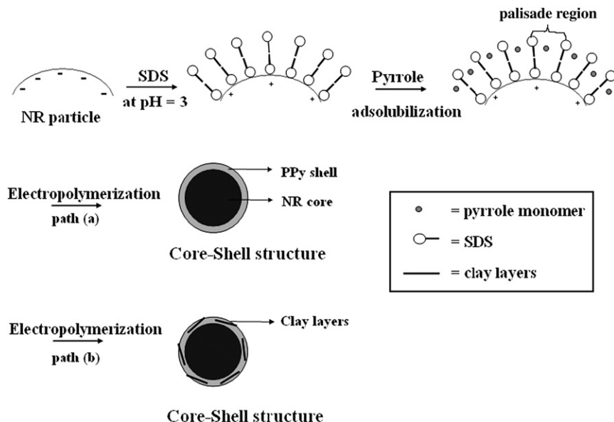
Fig. 3. Schematic of the formation mechanism of admicelled rubbers (path a) and the nanocomposites (path b).
