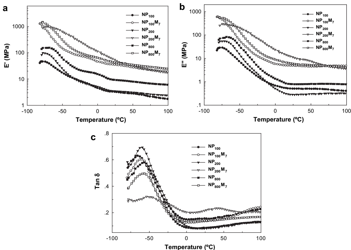
Fig. 11. Temperature dependence of the (a) storage modulus, (b) loss modulus, and (c) loss tangent of \text{NP}_x and the corresponding nanocomposites.
