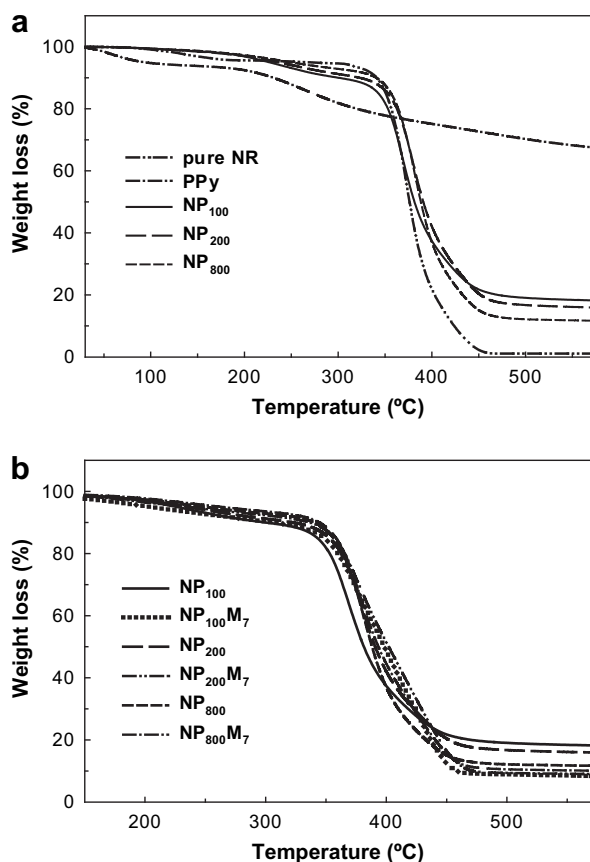
Fig. 12. TGA curves of (a) pure NR, PPy, and \text{NP}_x composites, and (b) \text{NP}_x and \text{NP}_x\text{M}_7 nanocomposites.
