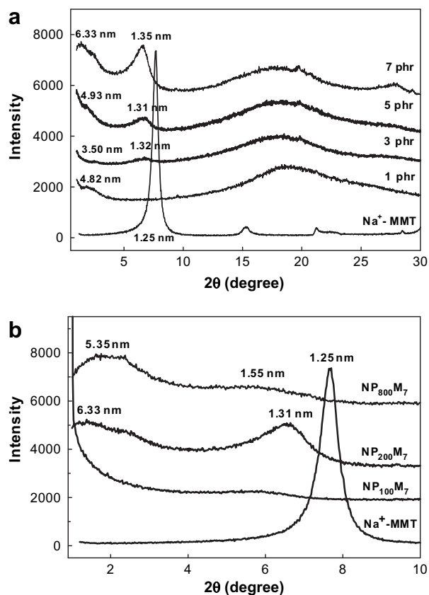
Fig. 4. XRD patterns of (a) \text{Na}^+ -MMT and \text{NP}_{200}\text{M}_y series, and (b) \text{Na}^+ -MMT and \text{NP}_x\text{M}_7 nanocomposites.
