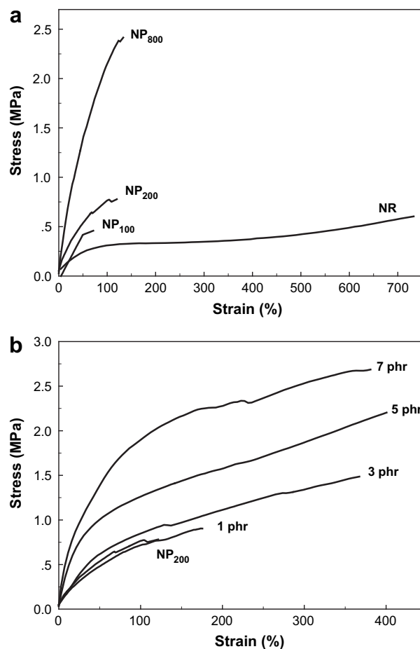
Fig. 9. Typical stress-strain curves of (a) pure NR and NP x composites, and (b) NP 200 M y and NP 800 M y series.
