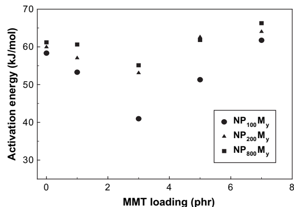
Fig. 15. Variation of the calculated activation energy of the nanocomposites with clay loading.
