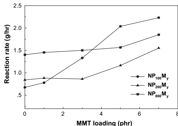
Fig. 5. Variation of polymerization rate of the nanocomposites with the clay loading.
