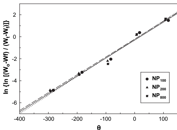
Fig. 14. Plots of \ln \{ \ln [(W_0 - W_f)/(W_t - W_f)] \} against \theta .
