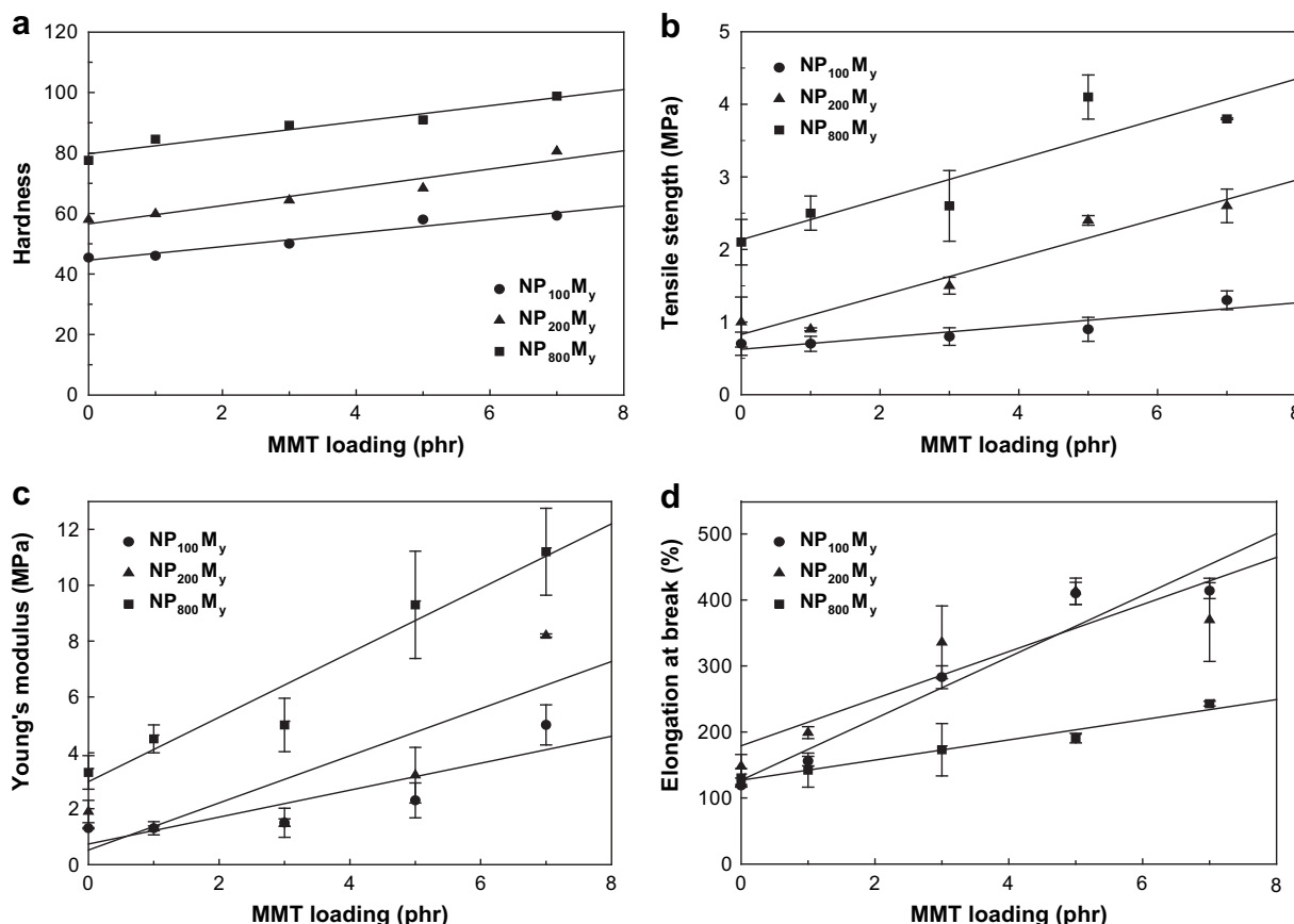
Fig. 10. Dependence of the mechanical properties of the NP 100 M y , NP 200 M y , and NP 800 M y series on clay loading: (a) hardness, (b) tensile strength, (c) Young's modulus, and (d) elongation at break.
