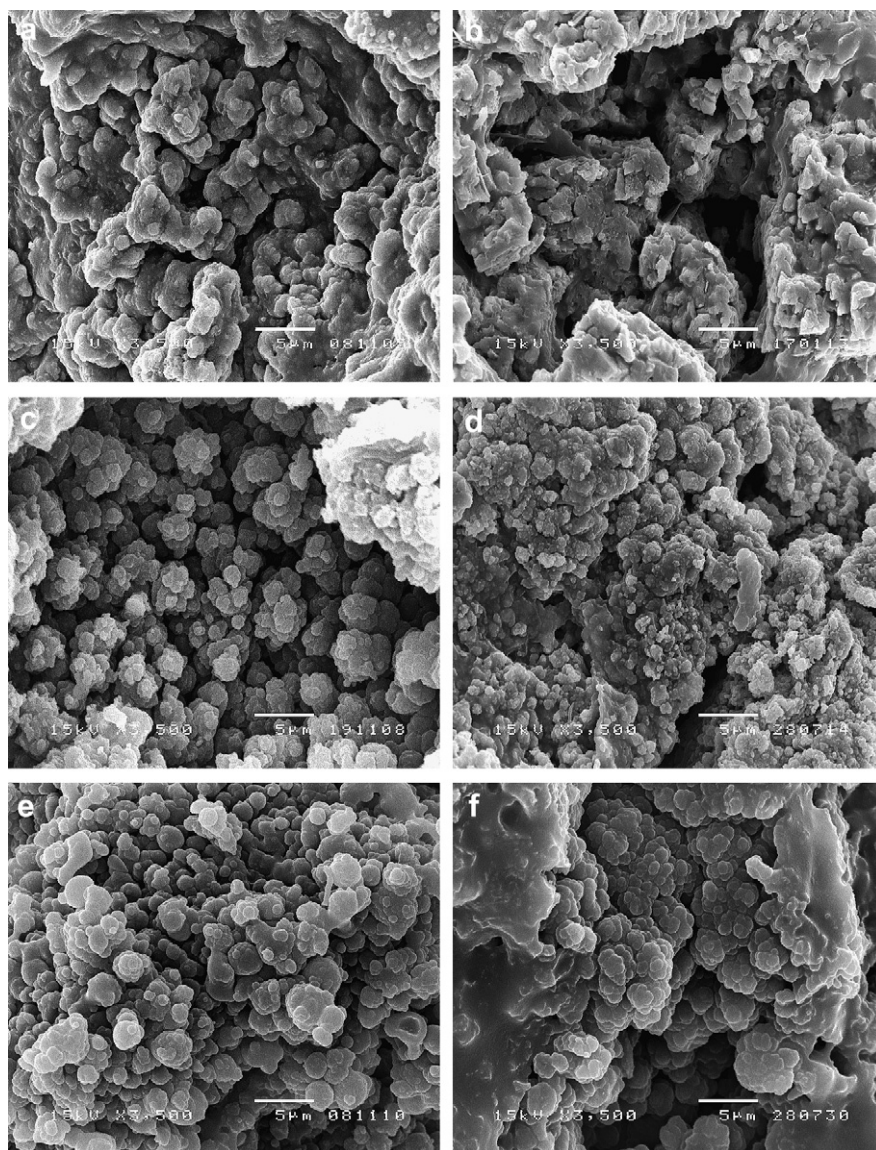
Fig. 2. SEM micrographs of (a) \text{NP}_{100} , (c) \text{NP}_{200} , and (e) \text{NP}_{800} , with the corresponding nanocomposites (b) \text{NP}_{100}\text{M}_7 , (d) \text{NP}_{200}\text{M}_7 , and (f) \text{NP}_{800}\text{M}_7 at the same magnification ( \times 3500 ).
