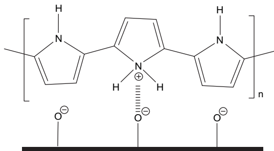
Fig. 7. Electrostatic interaction between a protonated PPy chain and the clay layer.
